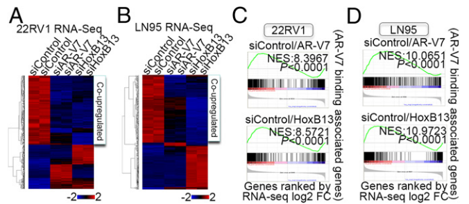
Fig. 3. HoxB13 and AR-V7 coup-regulate diverse target oncogenes in CRPC. (A and B) Heatmaps of regulated genes (FDR < 0.05, fold-change > 2) after AR-V7 or HoxB13 silencing in 22RV1 (A) and LN95 cells (B). (C and D) GSEA analyses compare associated genes within \pm 50 kb of AR-V7 binding locations with AR-V7 or HoxB13 regulated genes determined by RNA-seq analysis in 22RV1 (C) and LN95 (D) cells.
